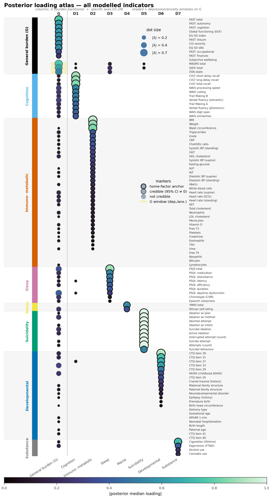
Figure F2: The complete posterior loading atlas. As Figure 2a but showing every modelled indicator (all 88 continuous and explicit items) grouped by home factor, with no per-block cap. Dot size and colour encode the absolute posterior median loading; outlined dots have a 95% credible interval excluding zero (heavier ring = home-factor anchor). Three earned cross-loadings render as outlined dots in the cognition column—childhood adversity (CTQ-37, -0.094 ) and two poor-sleep items (PSQI latency +0.057 , PSQI daytime dysfunction -0.070 ), each with a 95% credible interval excluding zero. The diagonal block structure—each clinical block loading cleanly on its own specific axis, with a sparse general-burden ( G ) column—is the full anatomy of the measurement model summarised in the main-text Figure 2.
