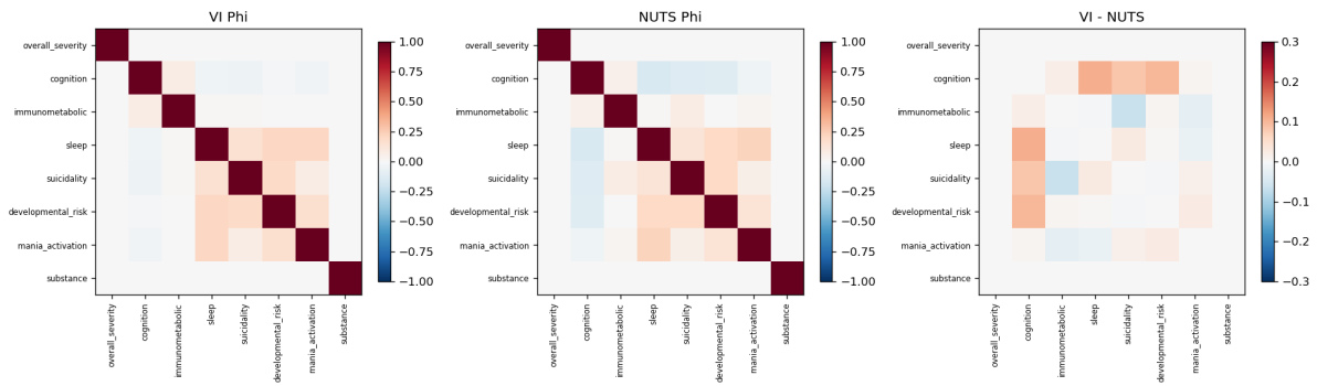
Figure H9: Inter-factor correlation \Phi : structure reproduced, magnitudes attenuated. Variational \Phi (left), NUTS \Phi (middle), and their difference (right). The block-diagonal orthogonality ( G , substance) is exact in both and the correlated specific block is positive in both; the difference panel localizes the \sim 21\% attenuation to the small cognition cross-correlations.
