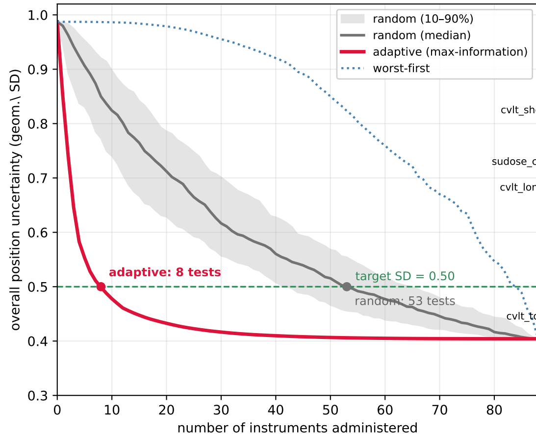
A Choosing the next test by information reaches the same precision in far fewer instruments
