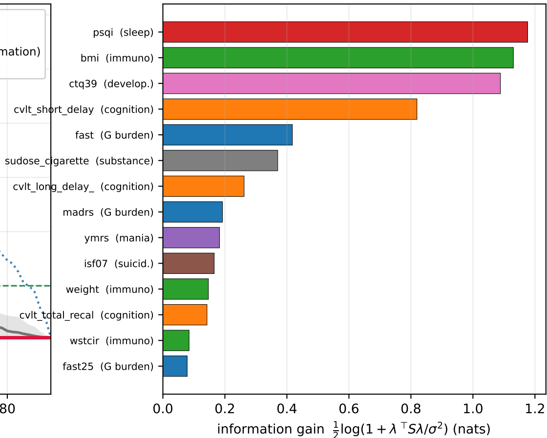
B The adaptive battery diversifies across axes (pick #1...#14, coloured by home factor)
