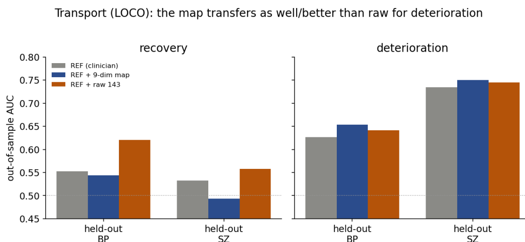
Figure 34. Leave-one-cohort-out transport (out-of-sample AUC on the held-out cohort). For deterioration the nine-dim map transfers as well or better than the 143 raw indicators; for recovery raw transfers better — the same target split as sufficiency.
