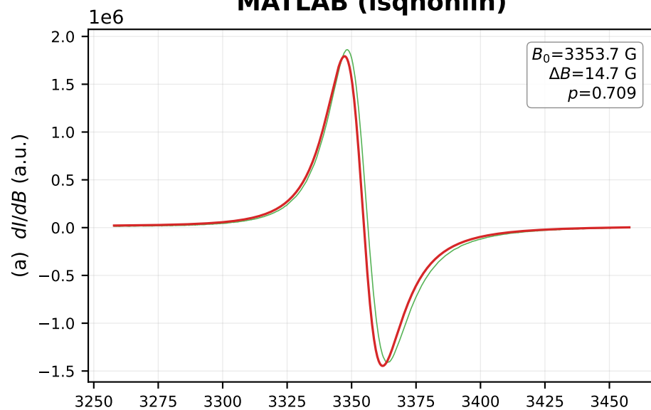
MATLAB (lsqnonlin)
