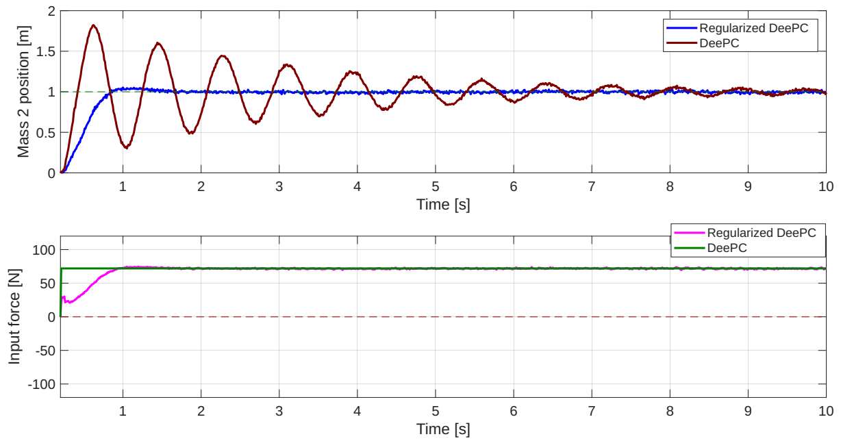
Figure 5.6: Regularized DeePC vs. DeePC; Noisy measurement LTI system
