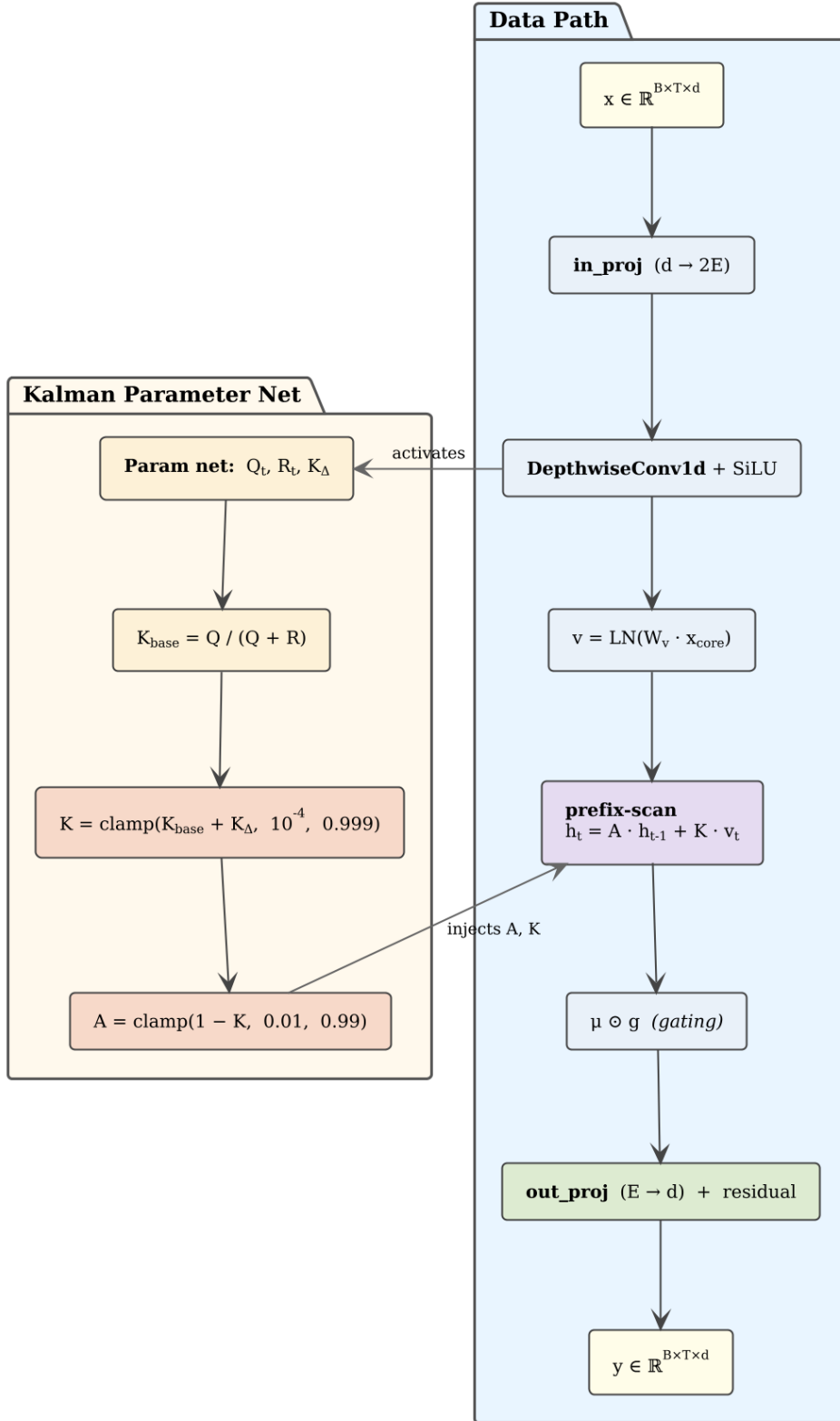
Figure 3.1: Full data-flow diagram of the KCMamba block. Yellow blocks ( Q_{net} , R_{net} , K_{net} ) learn the Kalman statistics. The purple block performs the parallel prefix-scan on GPU in O(\log T) synchronisation steps, and green blocks denote input/output projections.
