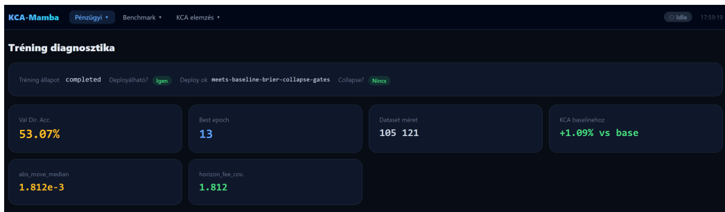
Figure 5.4: Offline training dashboard. The full training run can be monitored, including early-stopping status.
