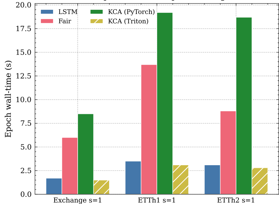
(b) Epoch times (5-epoch average)
