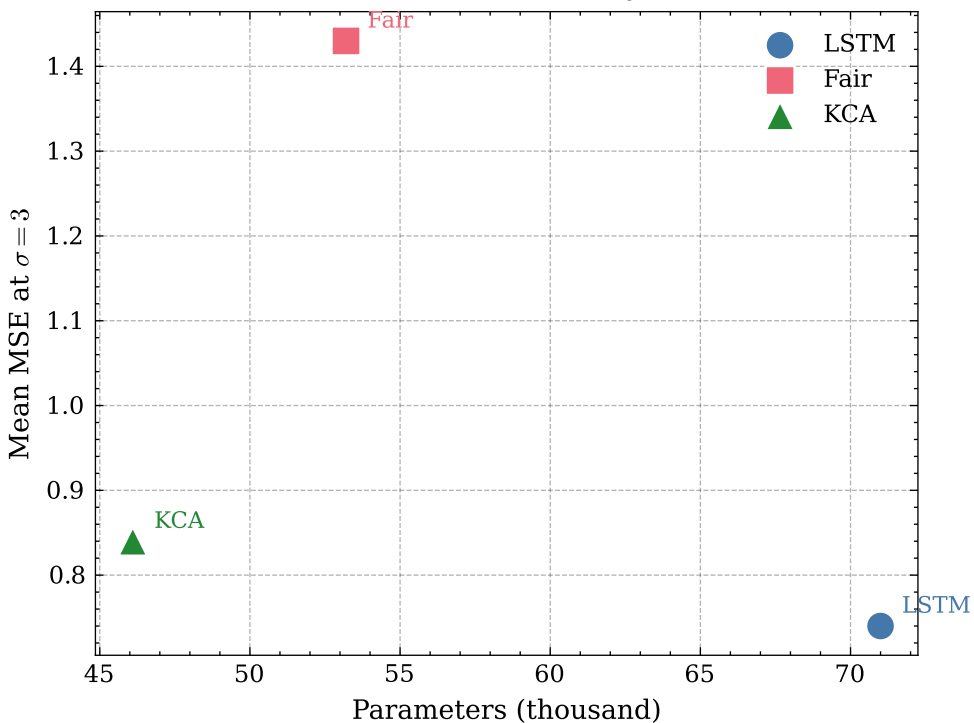
(a) Parameter efficiency ( \sigma = 3 )
