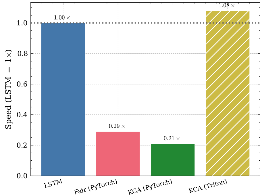
(b) Relative speed (LSTM = 1 \times )
