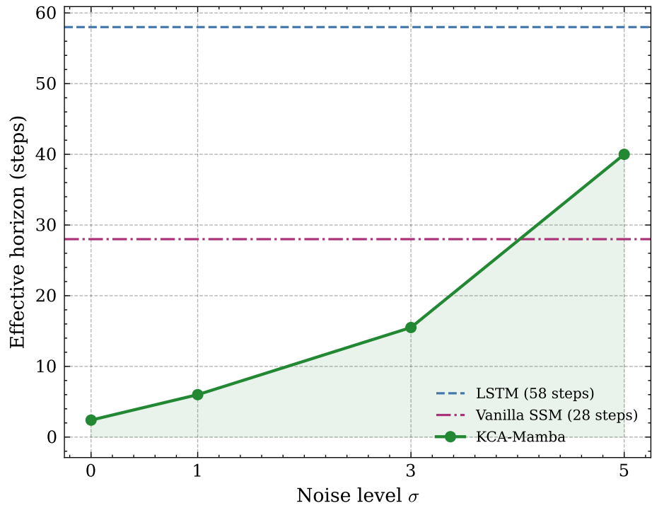
(b) Effective memory horizon ( A^k < 0.05 )
