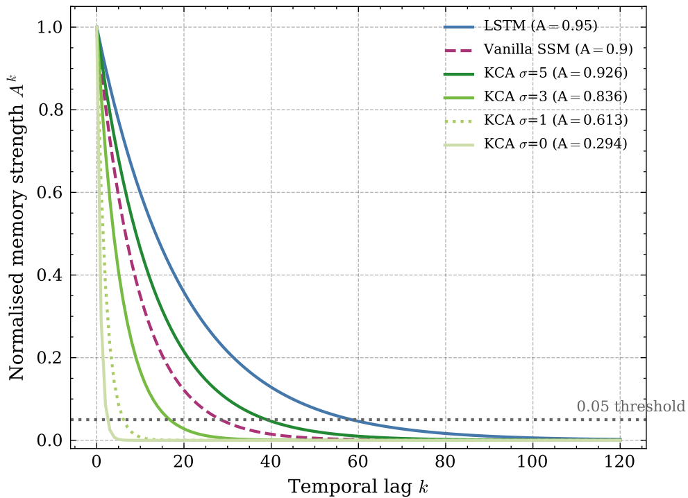
(a) Impulse response: memory decay
