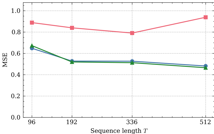
Exchange (daily) -- \sigma=3
