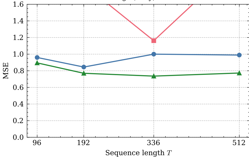
Exchange (daily) -- \sigma=3
