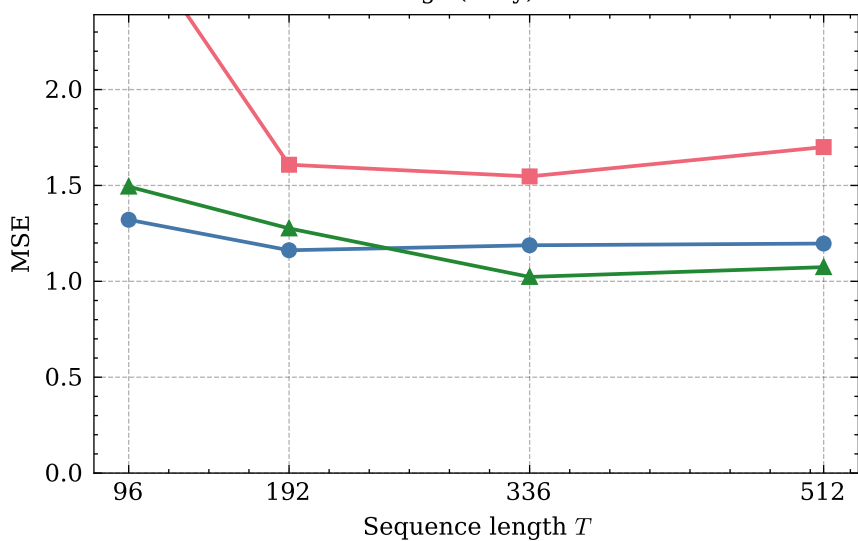
Exchange (daily) -- \sigma=5
