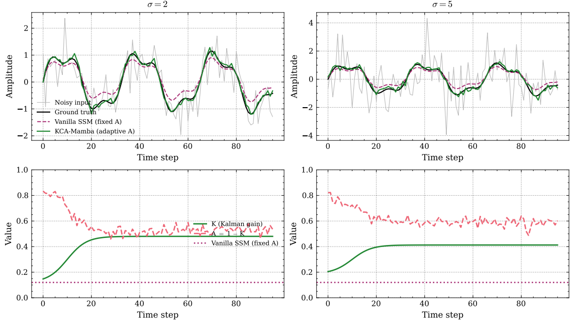
Figure 3.4: Synthetic signal filtering: vanilla SSM (standard Mamba, fixed A ) vs. KCMamba (adaptive K -gain) at moderate ( \sigma = 2 ) and strong ( \sigma = 5 ) noise. Top rows: predicted vs. true signal, where KCMamba tracks more tightly even under noise. Bottom rows: learned K values over time. Vanilla SSM has a fixed A , whereas KCMamba’s A adapts with noise level.
