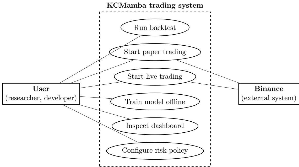
Figure 5.6: Use case diagram of the KCMamba system. The user has six main operations available; Binance participates as an external system on the paper- and live-trading paths (market data, order execution).
