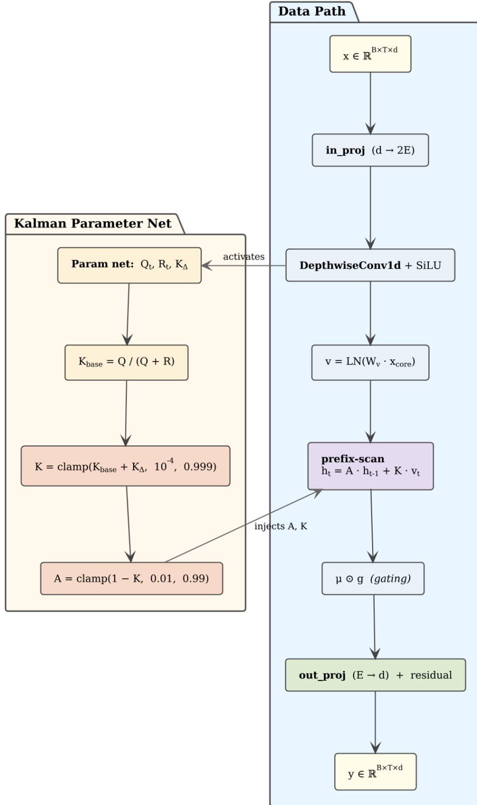
Figure 3.1: Full data-flow diagram of the KCMamba block. Yellow blocks ( Q_{net} , R_{net} , K_{net} ) learn the Kalman statistics. The purple block performs the parallel prefix-scan on GPU in O(\log T) synchronisation steps, and green blocks denote input/output projections.
