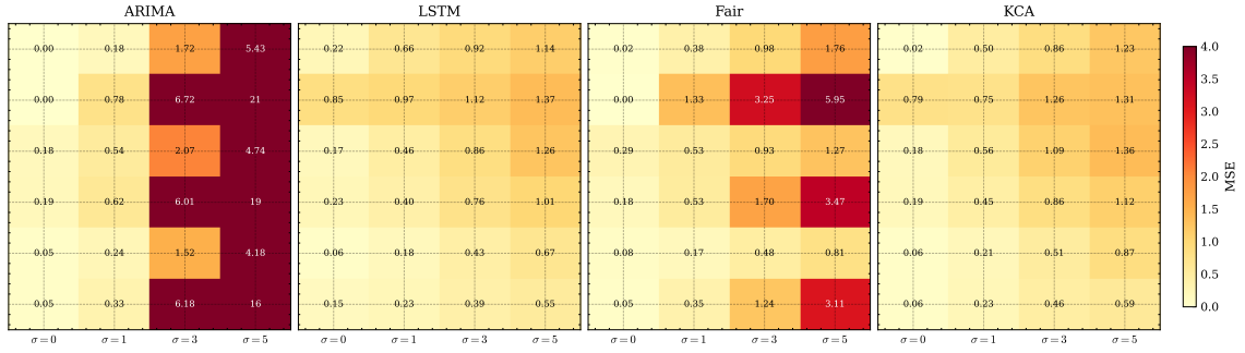
Figure 4.2: MSE heatmap for all four models (ARIMA, LSTM, Fair Mamba, KCMamba) across all configurations and noise levels. Dark red cells indicate catastrophic failure (MSE > 4). ARIMA and Fair Mamba collapse completely at s=16, \sigma \geq 3 , while KCMamba remains stable throughout.
