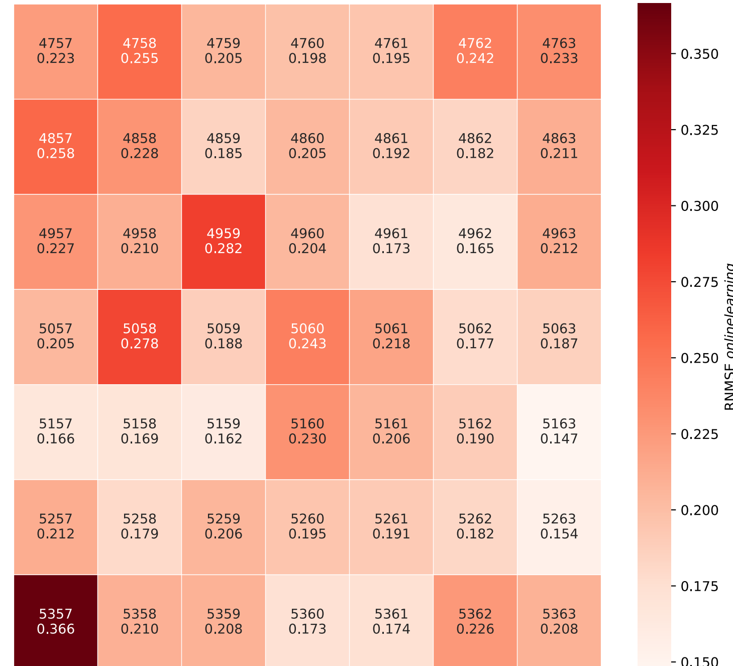
2CNN+LSTM
