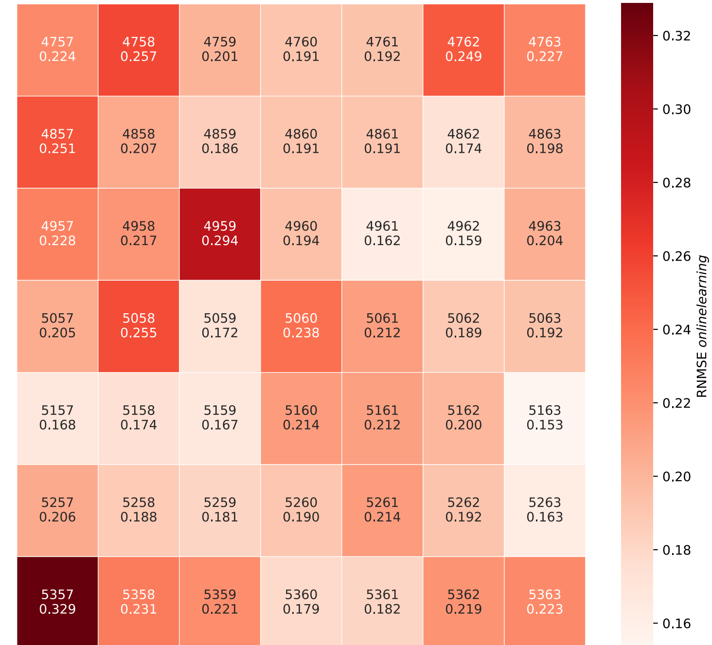
3CNN+LSTM
