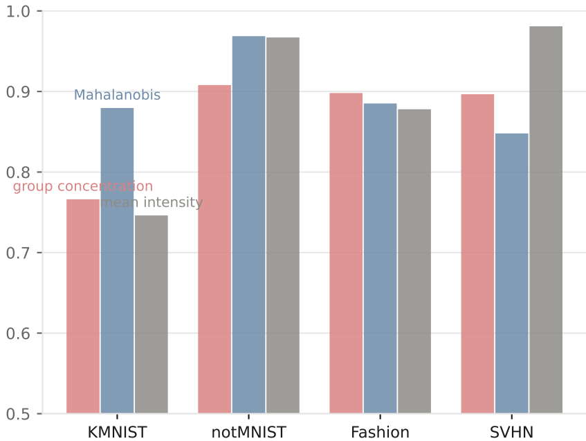
AUROC, MNIST vs out-of-distribution
