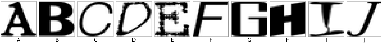
notMNIST
