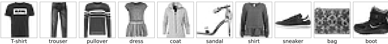
Fashion-MNIST
