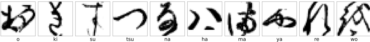
KMIST
