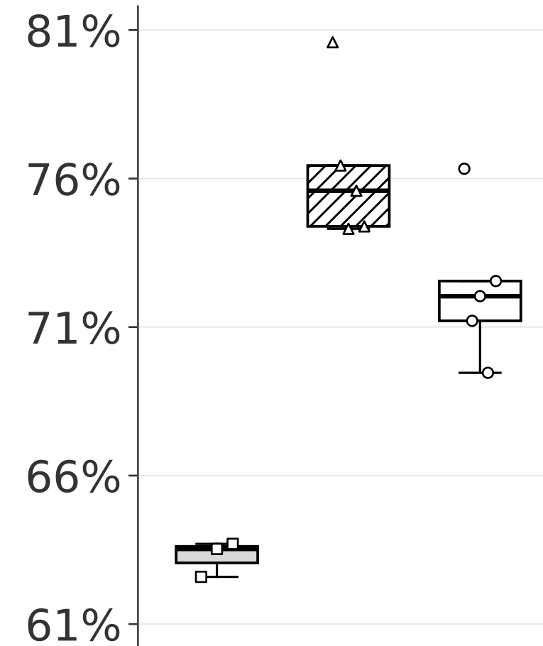
Fashion-MNIST
