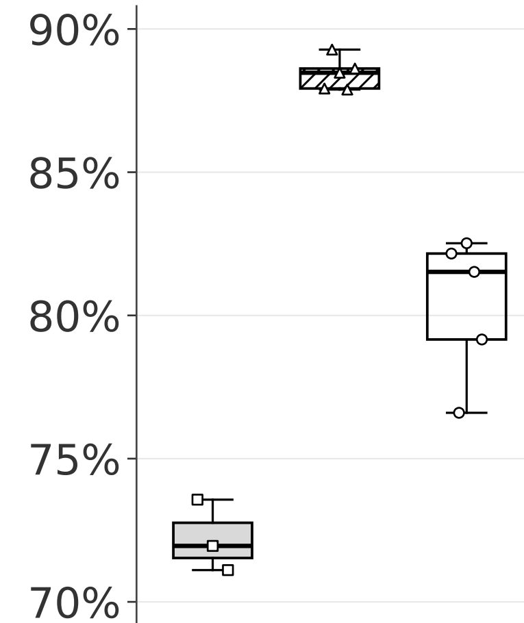
notMNIST
