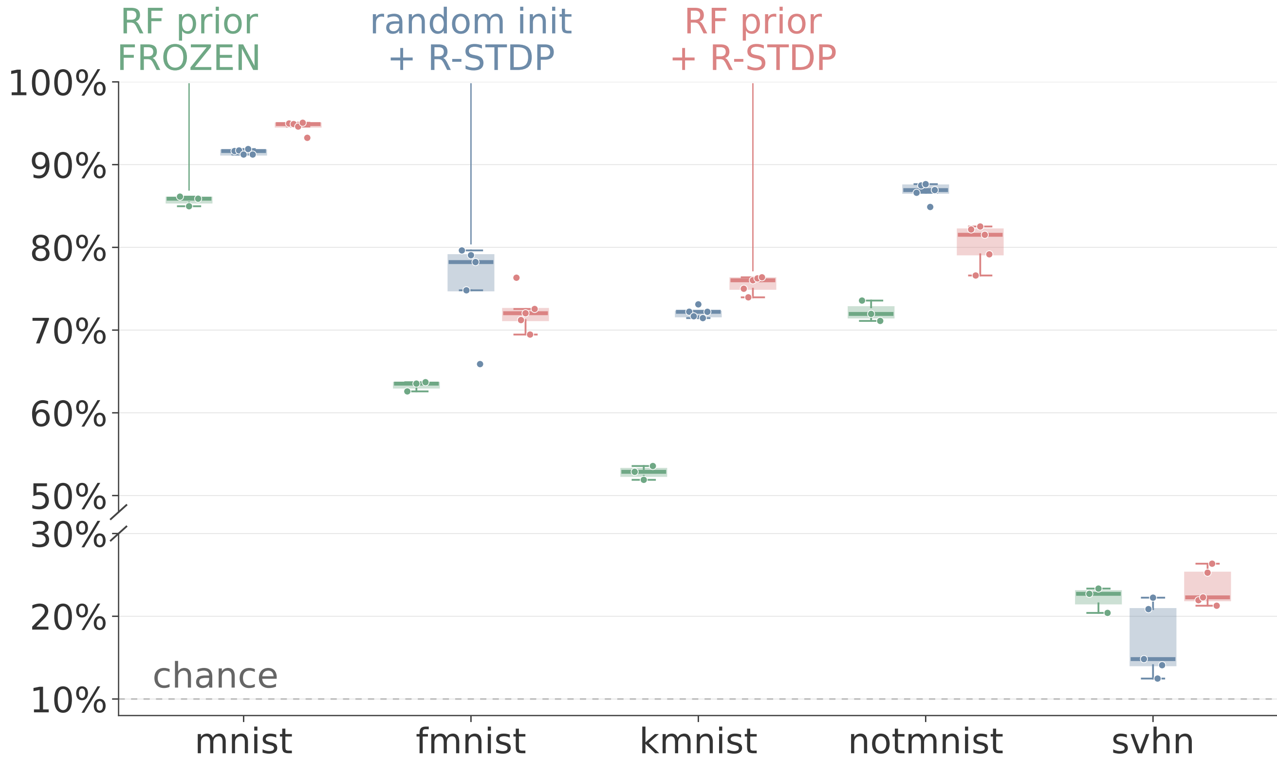
learned-readout test accuracy
