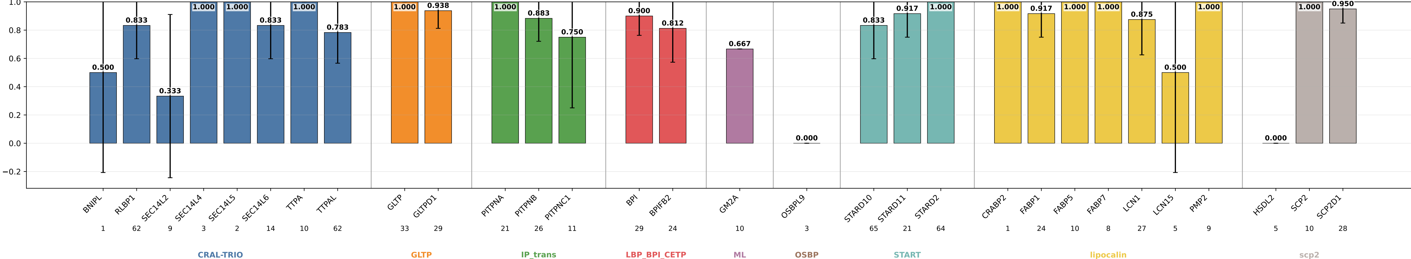
ge_s15_prothid32_hid64_noreg_adv sensitivity by subgroup ge_s15_prothid32_hid64_noreg_adv | class weights | lr=0.0001 | weight_decay=1e-05 | final_m=4 | final_dropout=0.0 | hiddim=64 | heads=8 | batch=16 | ep=120 | seeds=0,1,2,3,4
