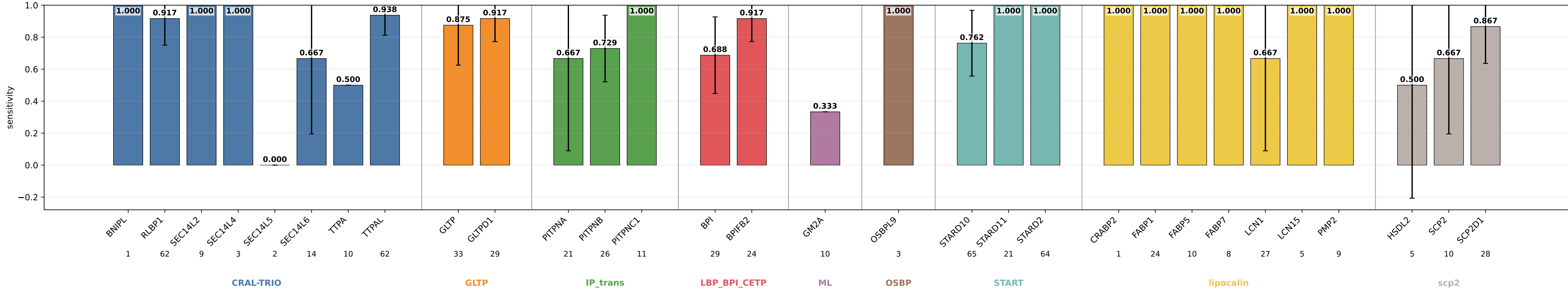
ge_s15_prothid32_hid64_noreg_attnpool sensitivity by subgroup ge_s15_prothid32_hid64_noreg_attnpool | class weights | lr=0.0001 | weight_decay=1e-05 | final_m=4 | final_dropout=0.0 | hiddim=64 | heads=8 | batch=16 | ep=120 | seeds=0,1,2,4
