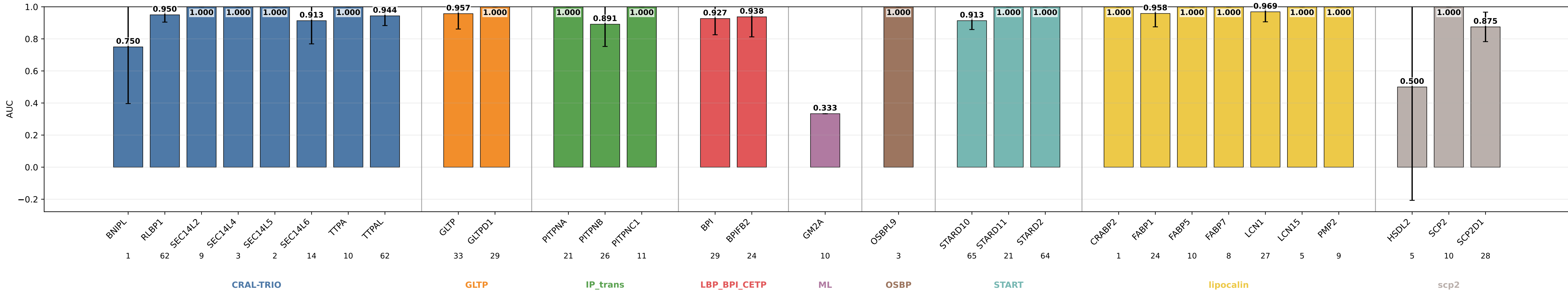
ge_s15_prothid32_hid64_noreg_doubleattn AUC by subgroup ge_s15_prothid32_hid64_noreg_doubleattn | class weights | lr=0.0001 | weight_decay=1e-05 | final_m=4 | final_dropout=0.0 | hiddim=64 | heads=8 | batch=16 | ep=120 | seeds=0,1,2,3,4
