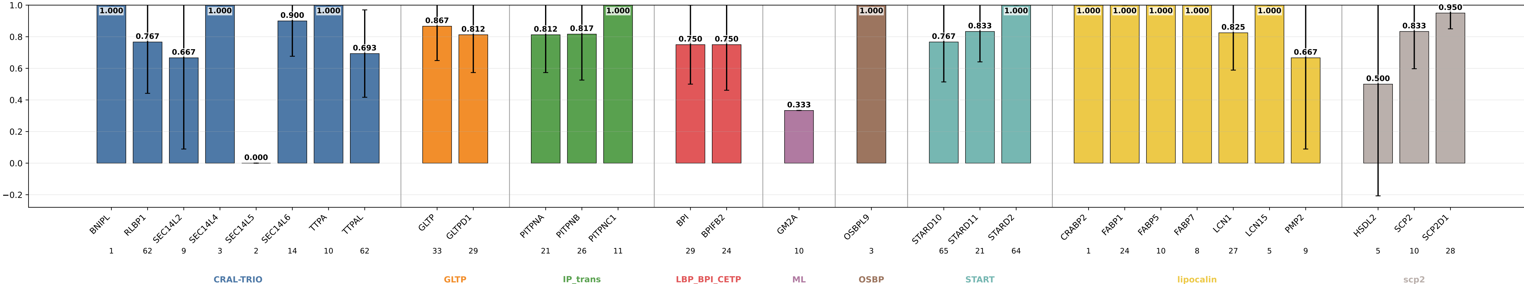
mlp_s15_nomb_hid32_m8_d21_experimental_lipid_volume sensitivity by subgroup mlp_s15_nomb_hid32_m8_d21_experimental_lipid_volume | class weights | lr=0.0001 | weight_decay=0.01 | final_m=4 | final_dropout=0.1 | hiddim=32 | heads=8 | batch=16 | ep=120 | seeds=0,1,2,3,4
