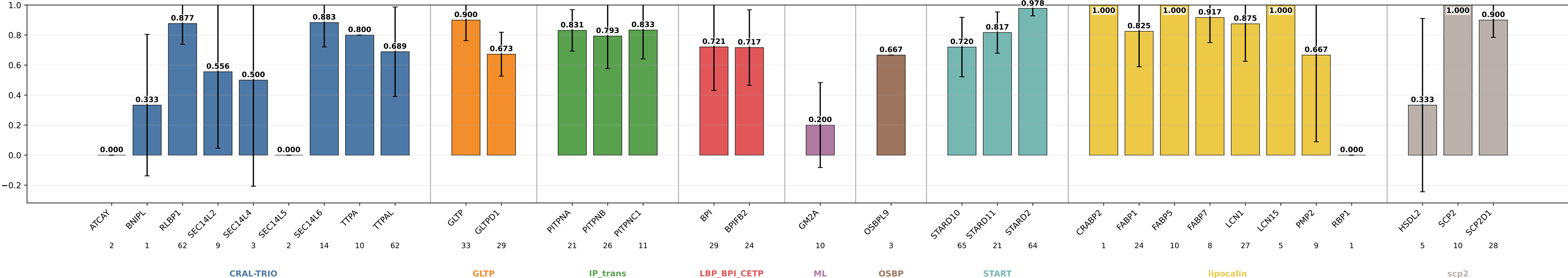
mlp_s15_nomb_hid32_m8_d21_pocket_free_volume F1 by subgroup mlp_s15_nomb_hid32_m8_d21_pocket_free_volume | class weights | lr=0.0001 | weight_decay=0.01 | final_m=4 | final_dropout=0.1 | hiddim=32 | heads=8 | batch=16 | ep=120 | seeds=0,1,2,3,4
