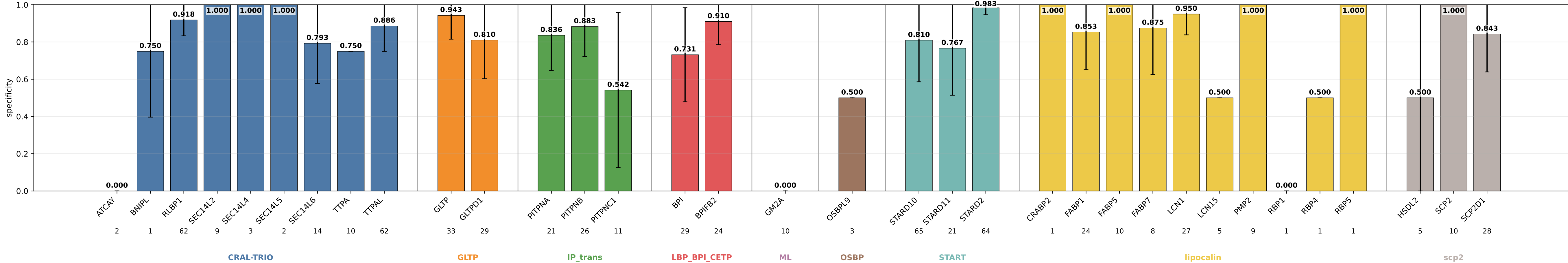
mlp_s15_nomb_hid32_m8_d21_volumes3 specificity by subgroup mlp_s15_nomb_hid32_m8_d21_volumes3 | class weights | lr=0.0001 | weight_decay=0.01 | final_m=4 | final_dropout=0.1 | hiddim=32 | heads=8 | batch=16 | ep=120 | seeds=0,1,2,3,4
