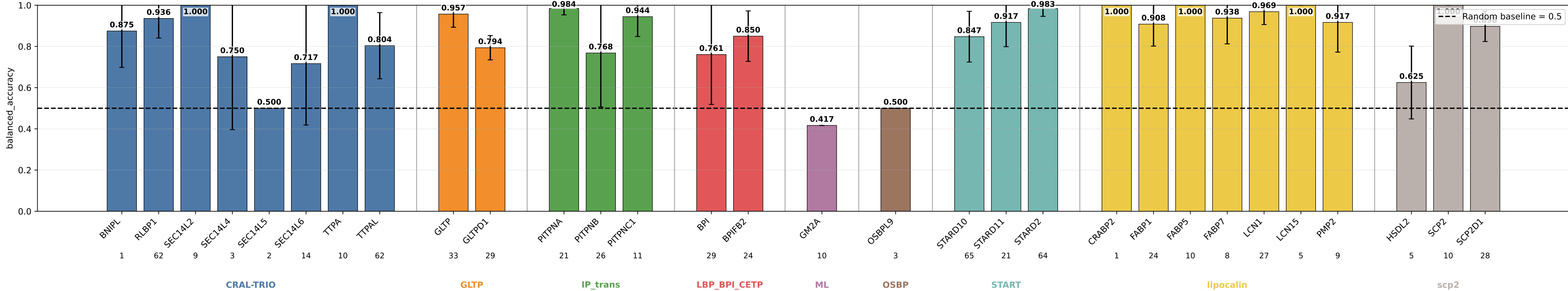
mlp_s15_nomb_hid64_3mlp balanced_accuracy by subgroup mlp_s15_nomb_hid64_3mlp | class weights | lr=0.0001 | weight_decay=0.01 | final_m=4 | final_dropout=0.1 | hiddim=64 | heads=8 | batch=16 | ep=120 | seeds=0,1,2,3,4
