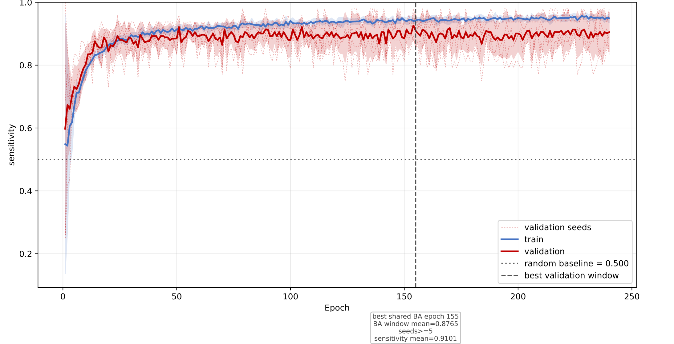
species15: mean sensitivity learning curve across seeds
