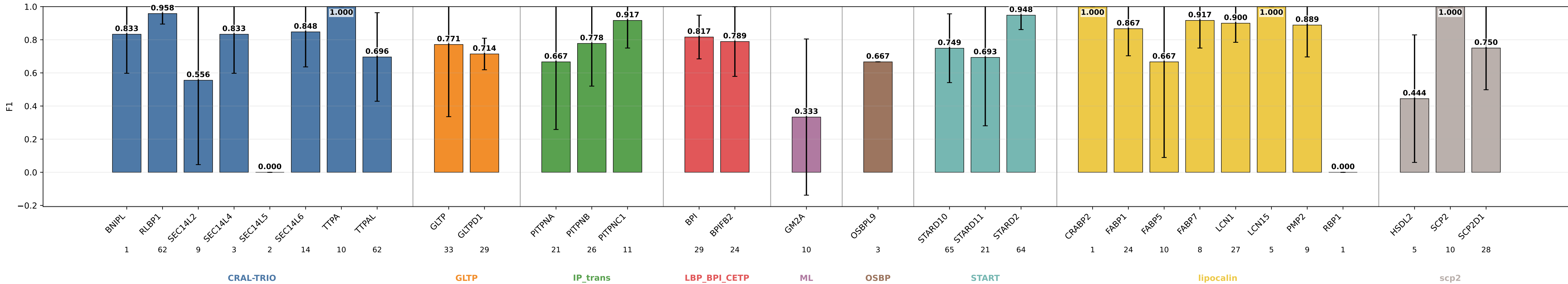
mlp_s15_nomb_hid64_ep360 F1 by subgroup mlp_s15_nomb_hid64_ep360 | class weights | lr=0.0001 | weight_decay=0.01 | final_m=4 | final_dropout=0.1 | hiddim=64 | heads=8 | batch=16 | ep=360 | seeds=0,1,2,3,4
