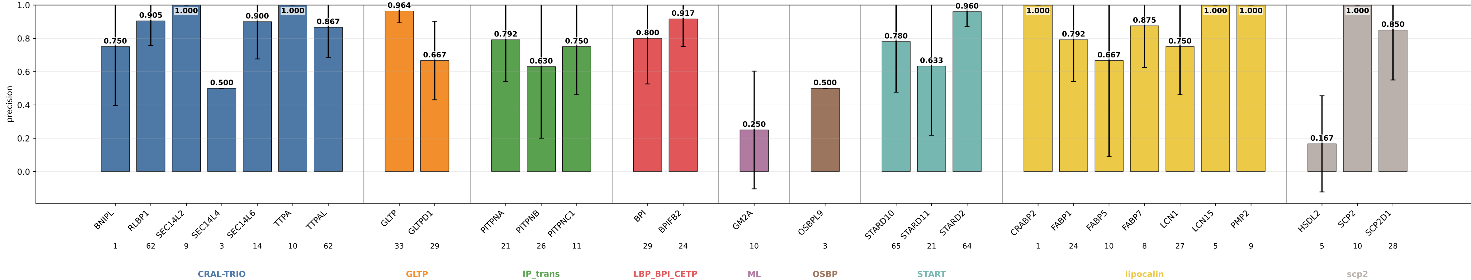
mlp_s15_nomb_hid64_pu005 precision by subgroup mlp_s15_nomb_hid64_pu005 | class weights | lr=0.0001 | weight_decay=0.01 | final_m=4 | final_dropout=0.1 | hiddim=64 | heads=8 | batch=16 | ep=120 | seeds=0,1,2,3,4
