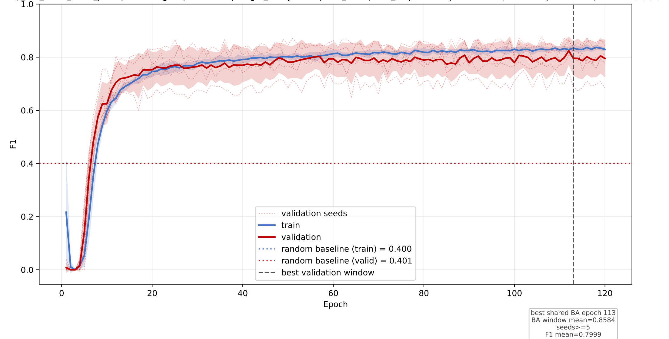
species15: mean F1 learning curve across seeds
