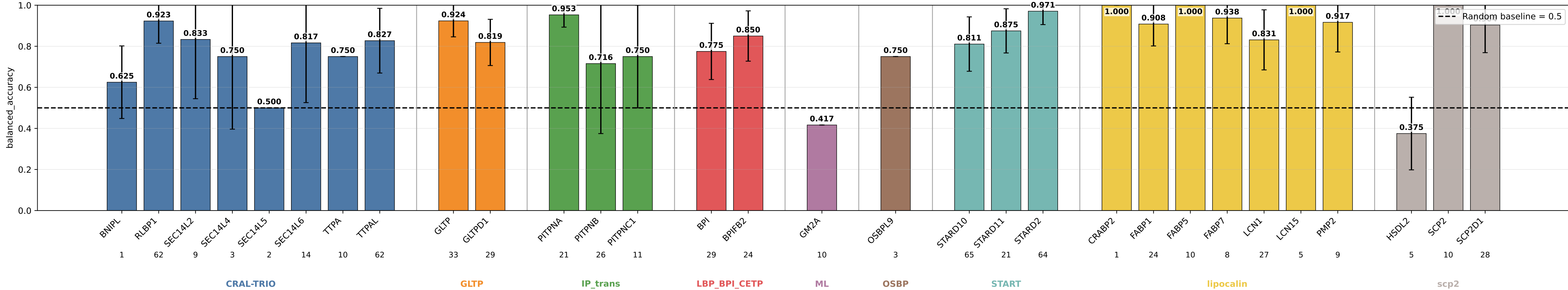
mlp_s15_nomb_hid64_pu01 balanced_accuracy by subgroup mlp_s15_nomb_hid64_pu01 | class weights | lr=0.0001 | weight_decay=0.01 | final_m=4 | final_dropout=0.1 | hiddim=64 | heads=8 | batch=16 | ep=120 | seeds=0,1,2,3,4
