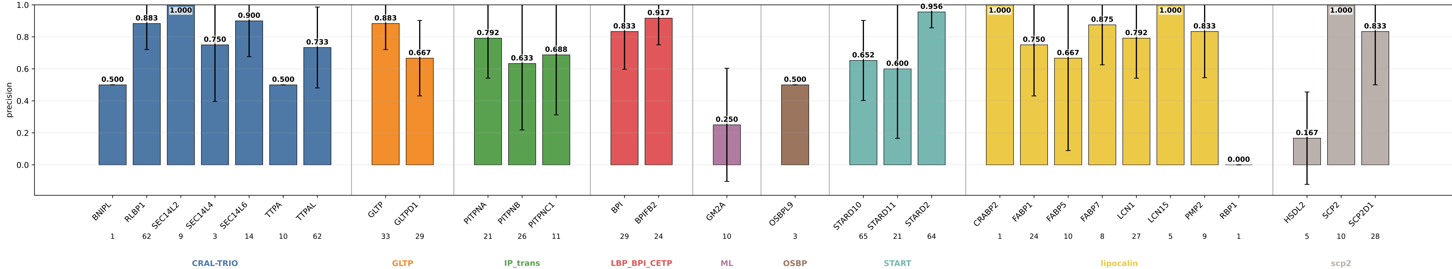
mlp_s15_nomb_hid64_pu01 precision by subgroup mlp_s15_nomb_hid64_pu01 | class weights | lr=0.0001 | weight_decay=0.01 | final_m=4 | final_dropout=0.1 | hiddim=64 | heads=8 | batch=16 | ep=120 | seeds=0,1,2,3,4
