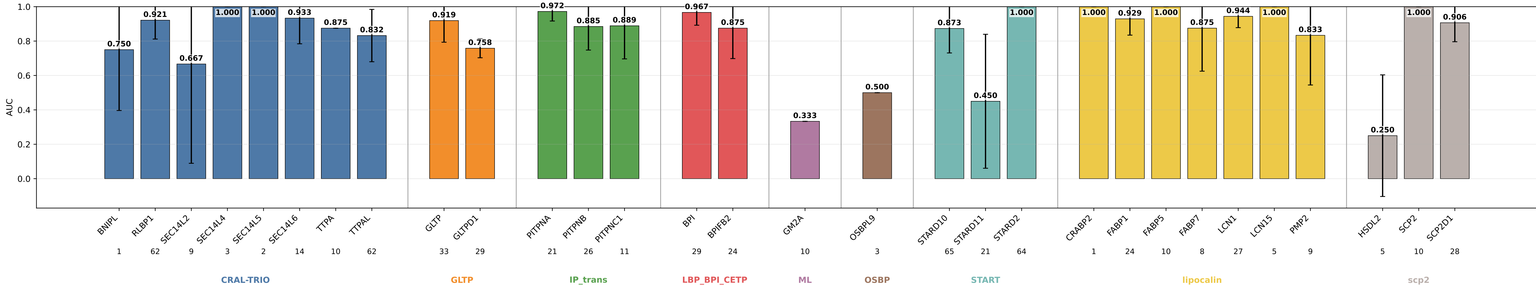
mlp_s15_nomb_hid64_pu01_subclass AUC by subgroup mlp_s15_nomb_hid64_pu01_subclass | class weights | lr=0.0001 | weight_decay=0.01 | final_m=4 | final_dropout=0.1 | hiddim=64 | heads=8 | batch=16 | ep=120 | seeds=0,1,2,3,4
