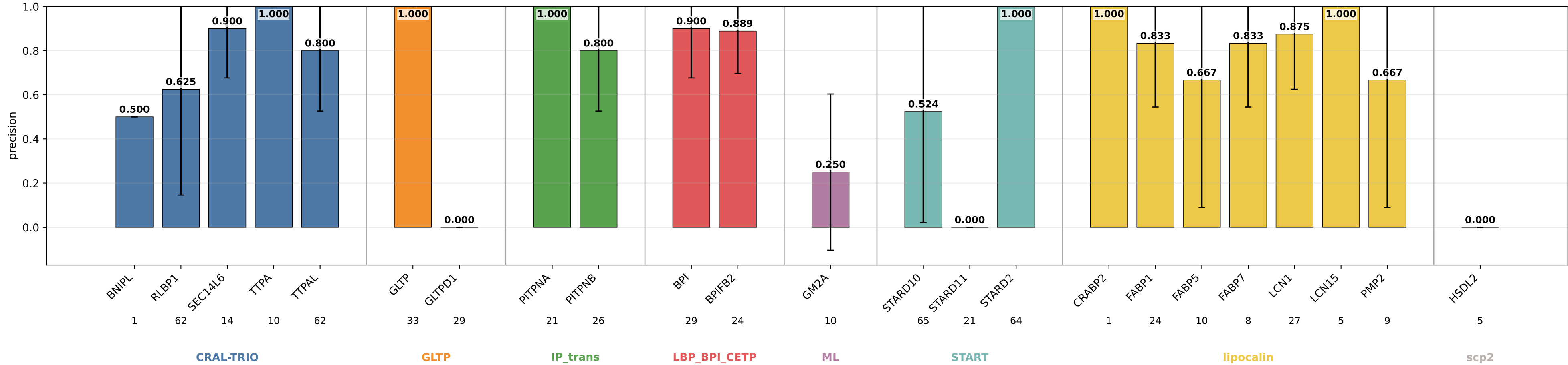
mlp_s15_nomb_hid64_pu01_subclass precision by subgroup mlp_s15_nomb_hid64_pu01_subclass | class weights | lr=0.0001 | weight_decay=0.01 | final_m=4 | final_dropout=0.1 | hiddim=64 | heads=8 | batch=16 | ep=120 | seeds=0,1,2,3,4
