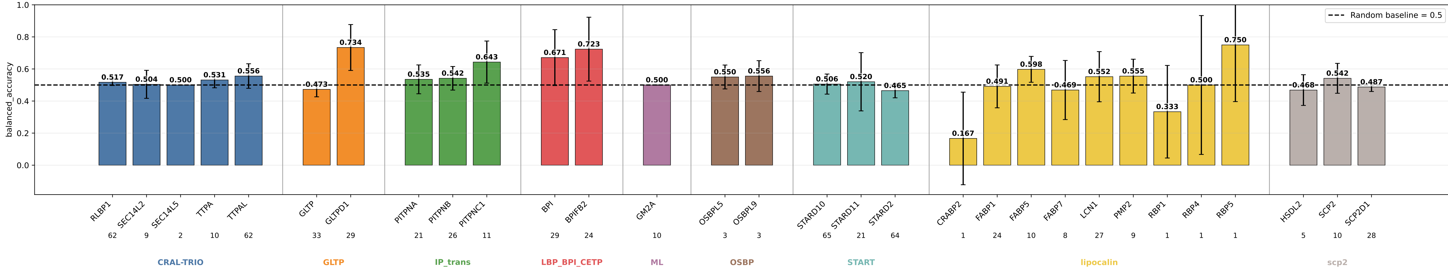
descriptors_head_family_neutral_lipprop_rankprot balanced_accuracy by subgroup descriptors_head_family_neutral_lipprop_rankprot | class weights | lr=0.0001 | weight_decay=0.01 | final_m=4 | final_dropout=0.1 | hiddim=8 | heads=8 | batch=32 | ep=120 | seeds=0,1,2,3,4
