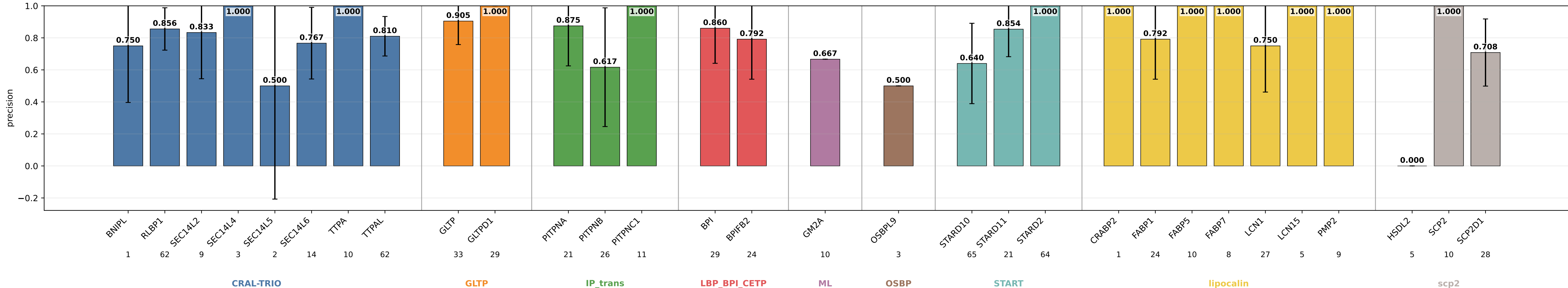
ge_s15_prothid32_hid64_noreg_prot64 precision by subgroup ge_s15_prothid32_hid64_noreg_prot64 | class weights | lr=0.0001 | weight_decay=1e-05 | final_m=4 | final_dropout=0.0 | hiddim=64 | heads=8 | batch=16 | ep=120 | seeds=0,1,2,3,4
