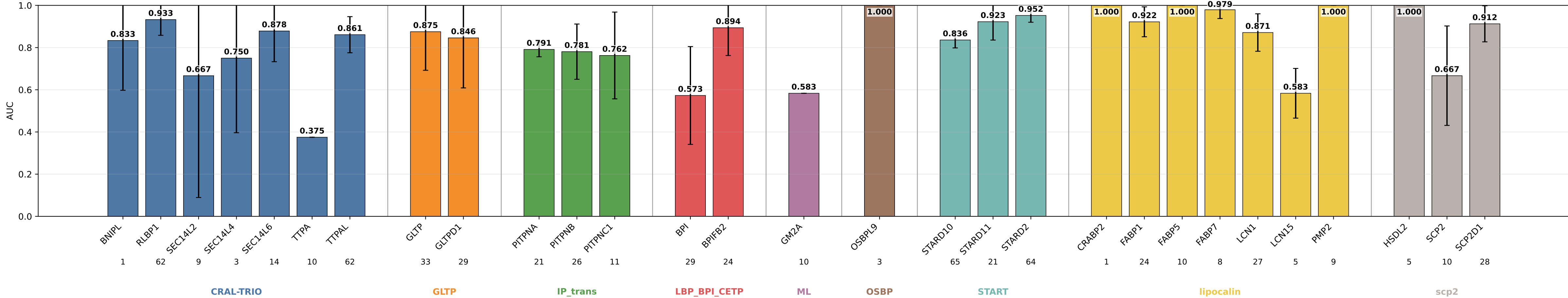
mlp_s15_mbw AUC by subgroup mlp_s15_mbw | class weights | lr=0.0001 | weight_decay=0.01 | final_m=4 | final_dropout=0.1 | hiddim=8 | heads=8 | batch=16 | ep=120 | seeds=0,1,2,3,4
