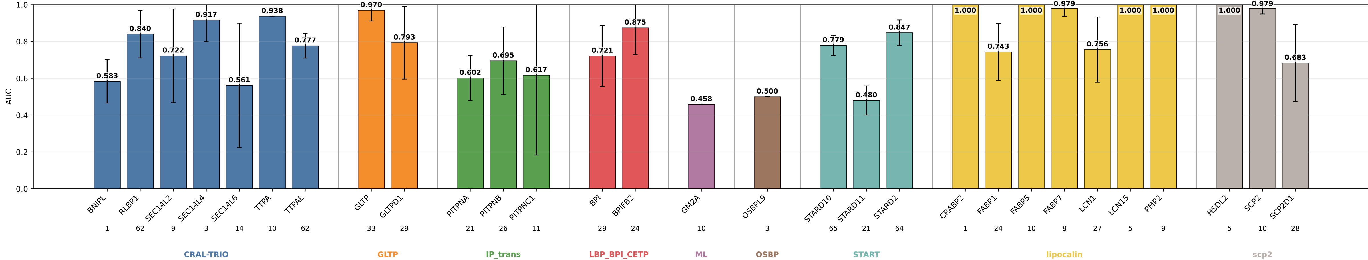
mlp_s15_mbw_hid32_d11 AUC by subgroup mlp_s15_mbw_hid32_d11 | class weights | lr=0.0001 | weight_decay=0.01 | final_m=4 | final_dropout=0.1 | hiddim=32 | heads=8 | batch=16 | ep=120 | seeds=0,1,2,3,4
