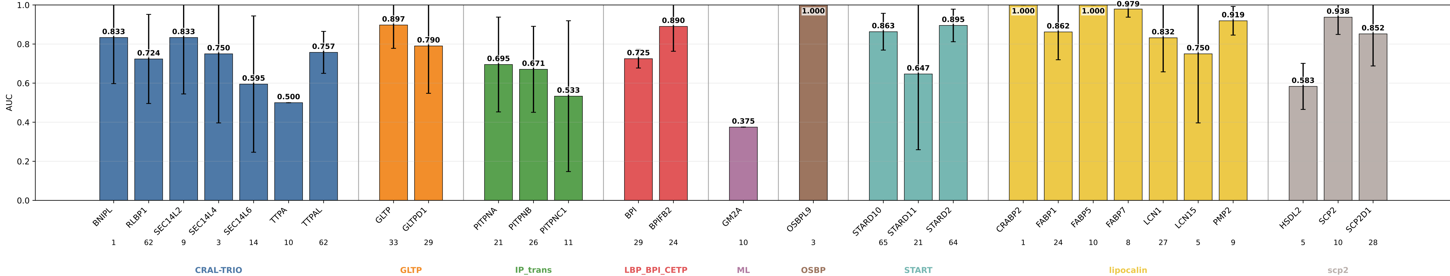
mlp_s15_mbw_hid32_d14 AUC by subgroup mlp_s15_mbw_hid32_d14 | class weights | lr=0.0001 | weight_decay=0.01 | final_m=4 | final_dropout=0.1 | hiddim=32 | heads=8 | batch=16 | ep=120 | seeds=0,1,2,3,4
