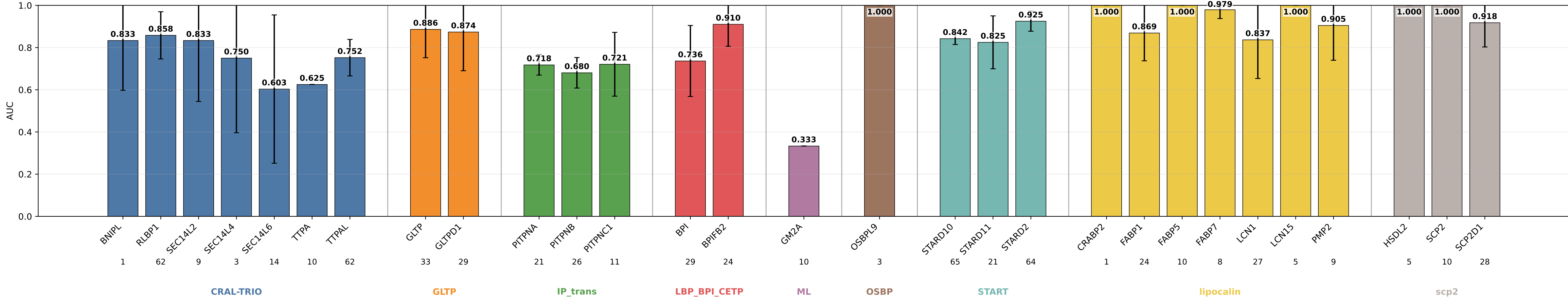
mlp_s15_mbw_hid32_d16 AUC by subgroup mlp_s15_mbw_hid32_d16 | class weights | lr=0.0001 | weight_decay=0.01 | final_m=4 | final_dropout=0.1 | hiddim=32 | heads=8 | batch=16 | ep=120 | seeds=0,1,2,3,4
