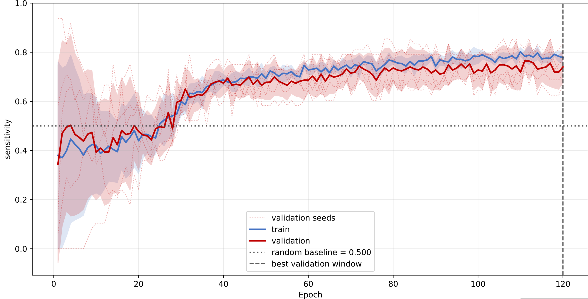
species15: mean sensitivity learning curve across seeds
