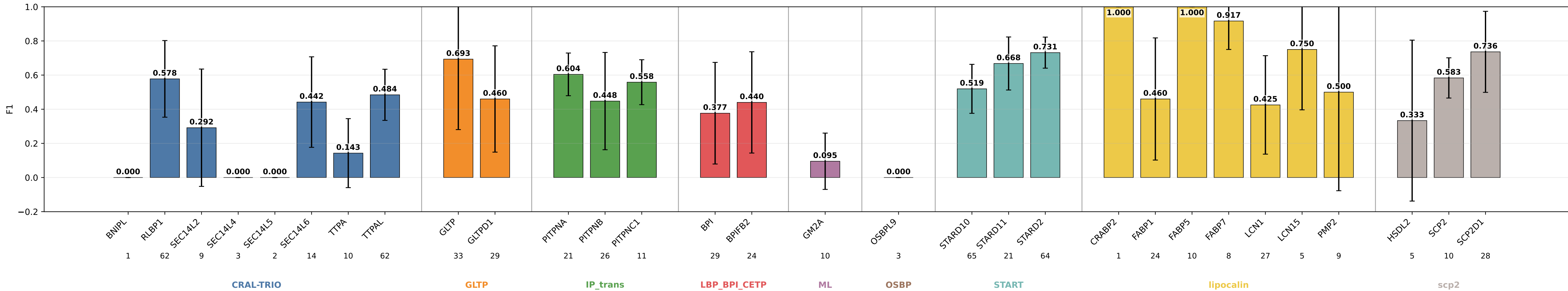
mlp_s15_mbw_hid32_d21 F1 by subgroup mlp_s15_mbw_hid32_d21 | class weights | lr=0.0001 | weight_decay=0.01 | final_m=4 | final_dropout=0.1 | hiddim=32 | heads=8 | batch=16 | ep=120 | seeds=0,1,2,3,4
