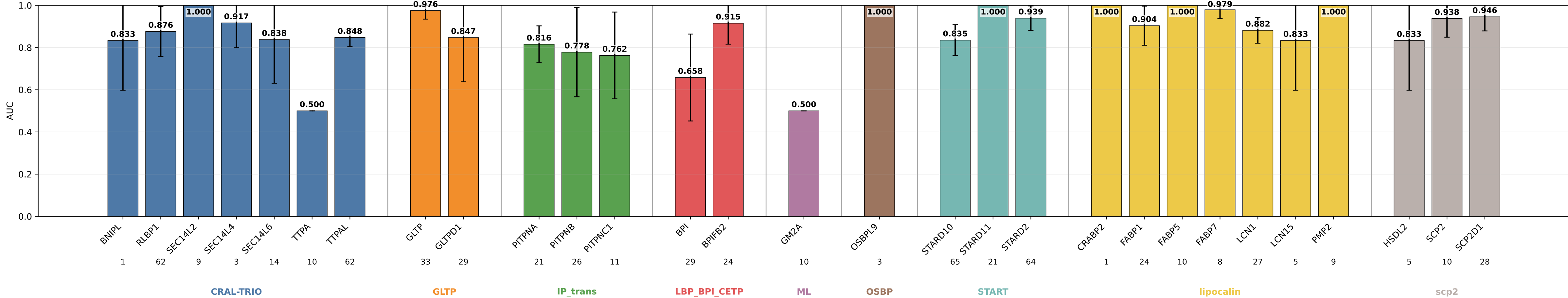
mlp_s15_mbw_hid32_d34 AUC by subgroup mlp_s15_mbw_hid32_d34 | class weights | lr=0.0001 | weight_decay=0.01 | final_m=4 | final_dropout=0.1 | hiddim=32 | heads=8 | batch=16 | ep=120 | seeds=0,1,2,3,4
