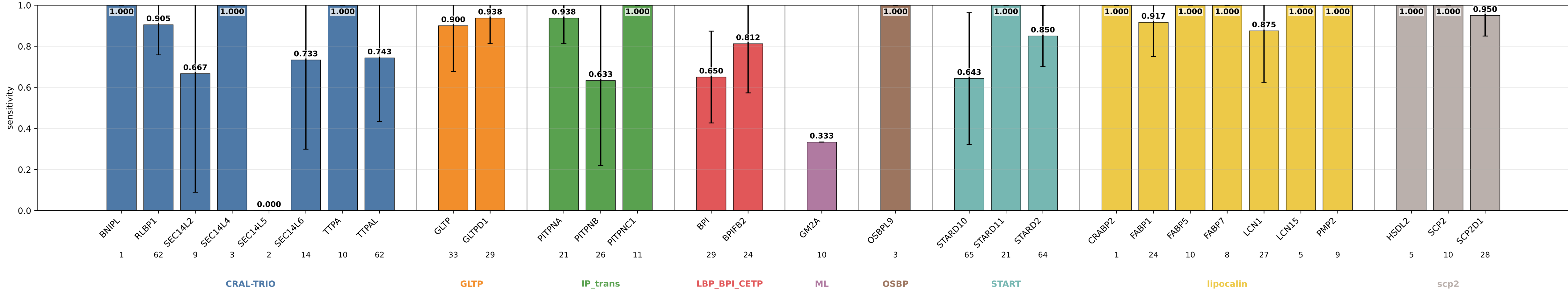
mlp_s15_mbw_hid32_lr3e4 sensitivity by subgroup mlp_s15_mbw_hid32_lr3e4 | class weights | lr=0.0003 | weight_decay=0.01 | final_m=4 | final_dropout=0.1 | hiddim=32 | heads=8 | batch=16 | ep=120 | seeds=0,1,2,3,4
