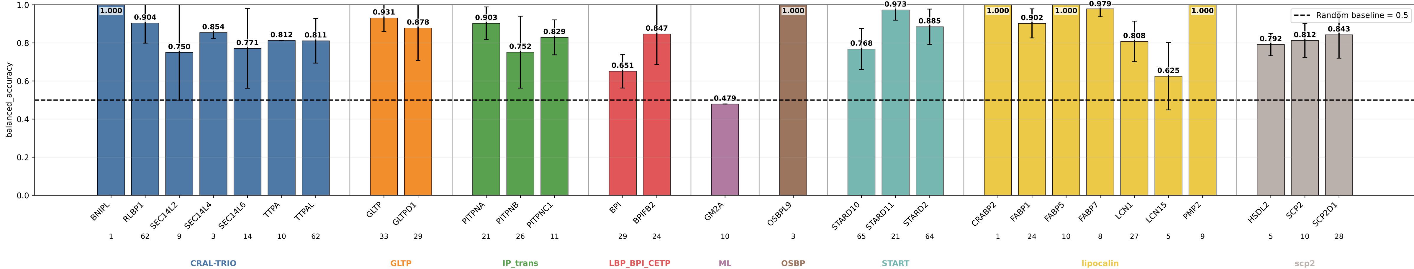
mlp_s15_mbw_hid32_m8 balanced_accuracy by subgroup mlp_s15_mbw_hid32_m8 | class weights | lr=0.0001 | weight_decay=0.01 | final_m=4 | final_dropout=0.1 | hiddim=32 | heads=8 | batch=16 | ep=120 | seeds=0,1,2,3,4
