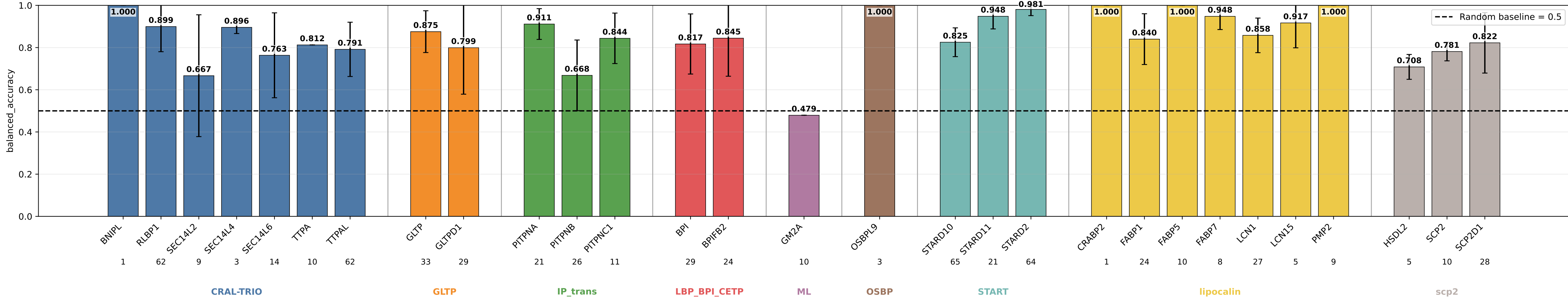
mlp_s15_nomb_hid32 balanced_accuracy by subgroup mlp_s15_nomb_hid32 | class weights | lr=0.0001 | weight_decay=0.01 | final_m=4 | final_dropout=0.1 | hiddim=32 | heads=8 | batch=16 | ep=120 | seeds=0,1,2,3,4
