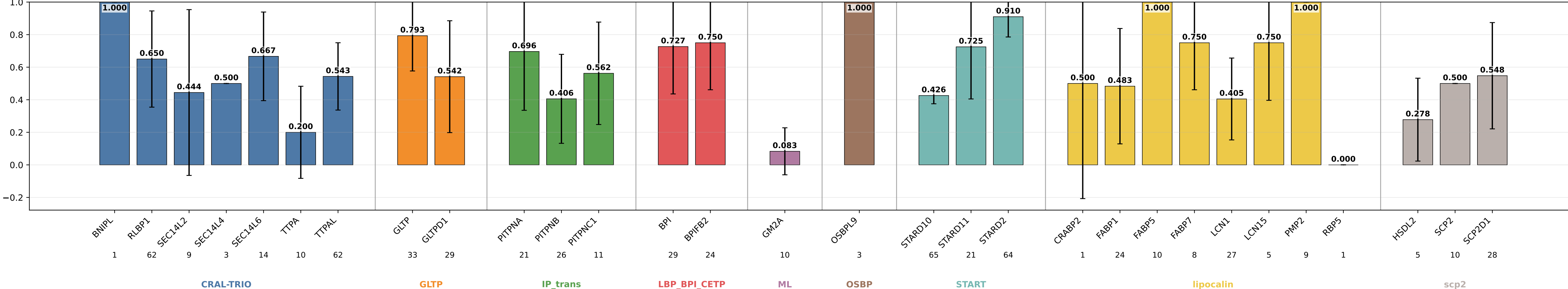
mlp_s15_nomb_hid32 precision by subgroup mlp_s15_nomb_hid32 | class weights | lr=0.0001 | weight_decay=0.01 | final_m=4 | final_dropout=0.1 | hiddim=32 | heads=8 | batch=16 | ep=120 | seeds=0,1,2,3,4
