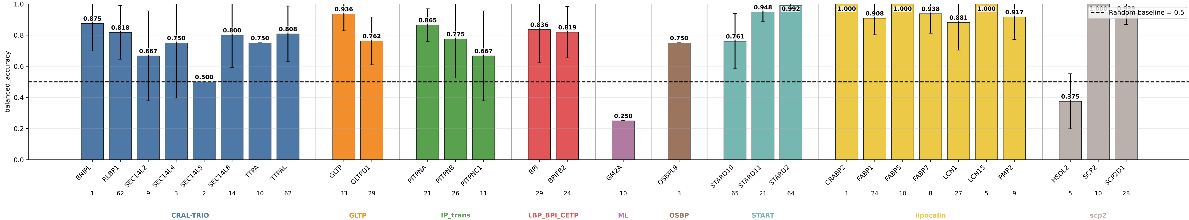
mlp_s15_nomb_hid32_m8_d34 balanced_accuracy by subgroup mlp_s15_nomb_hid32_m8_d34 | class weights | lr=0.0001 | weight_decay=0.01 | final_m=4 | final_dropout=0.1 | hiddim=32 | heads=8 | batch=16 | ep=120 | seeds=0,1,2,3,4
