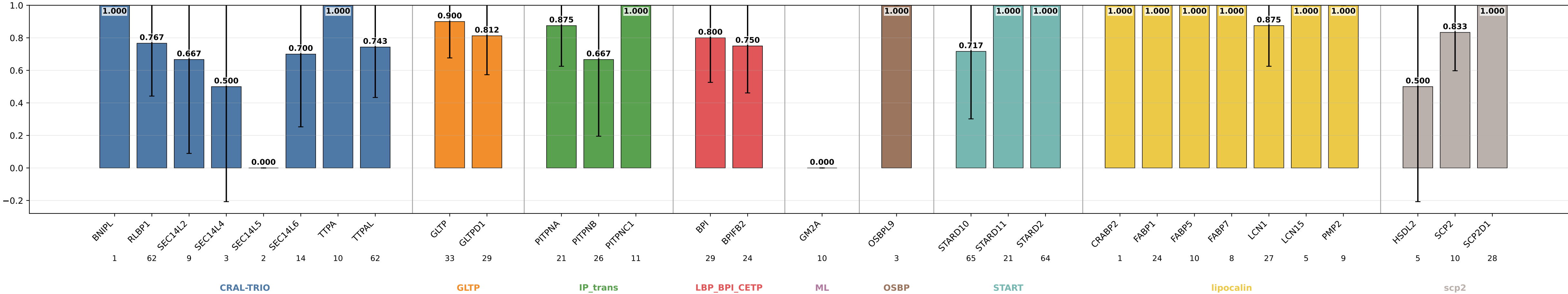
mlp_s15_nomb_hid32_m8_d34 sensitivity by subgroup mlp_s15_nomb_hid32_m8_d34 | class weights | lr=0.0001 | weight_decay=0.01 | final_m=4 | final_dropout=0.1 | hiddim=32 | heads=8 | batch=16 | ep=120 | seeds=0,1,2,3,4
